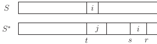
Figure 4.3: Schedules S and S^* for 1 | prec; pmtn; r_j | L_{\max} .
