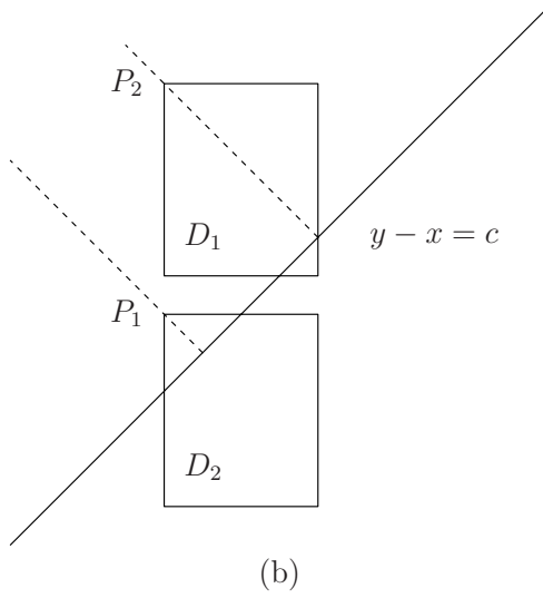
Figure 6.12: Ordering of intervals induced by obstacles on the sweep line. Case x_1 \leq x_2 .
