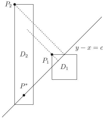
Figure 6.13: Ordering of intervals induced by obstacles on the sweep line. Case x_2 < x_1 .
